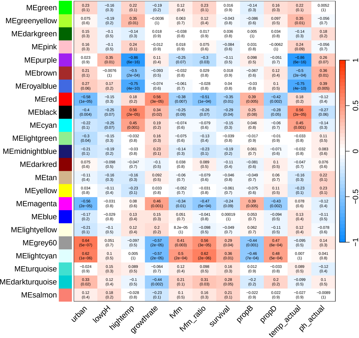
Module–trait relationships (raw)
